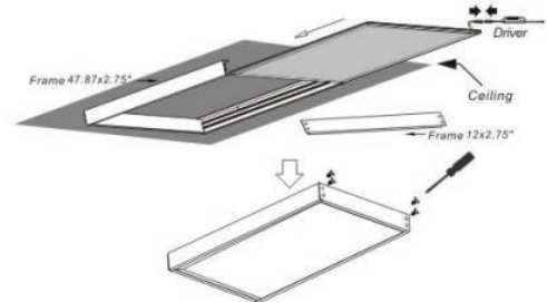
Surface Mounting Frame Kit
